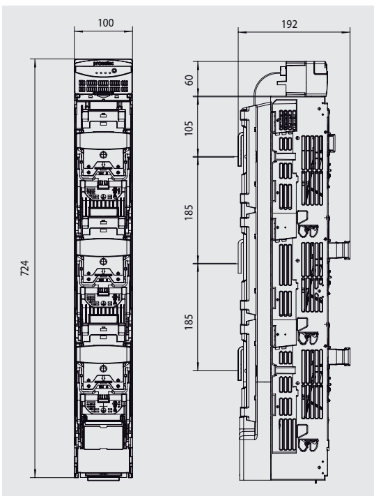
Fuse switch NH 1/2/3 (Type 438) + electronic FSC
